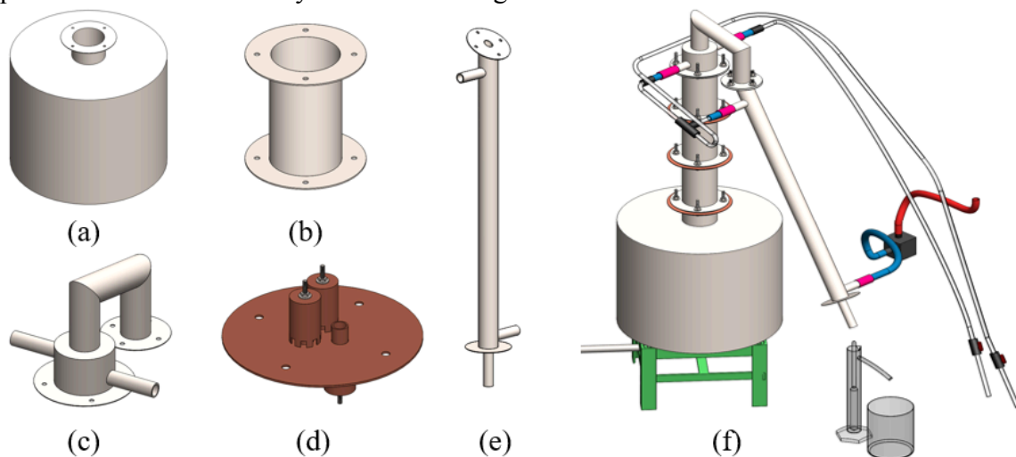
Figure 3. Computer-Aided Design (CAD) models of the components of the experimental setup: (a) Boiler, (b) Column unit, (c) Reflux condenser, (d) Bubble cap tray, (e) Main condenser, (f) Full assembly
