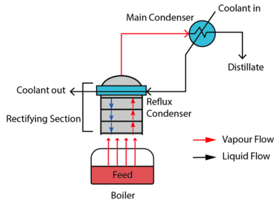
Figure 2. Schematic representation of the batch distillation apparatus, illustrating vapor flow from the boiler through the rectifying section and condensation in the reflux and main condensers, showing the resulting distillate and reflux streams
