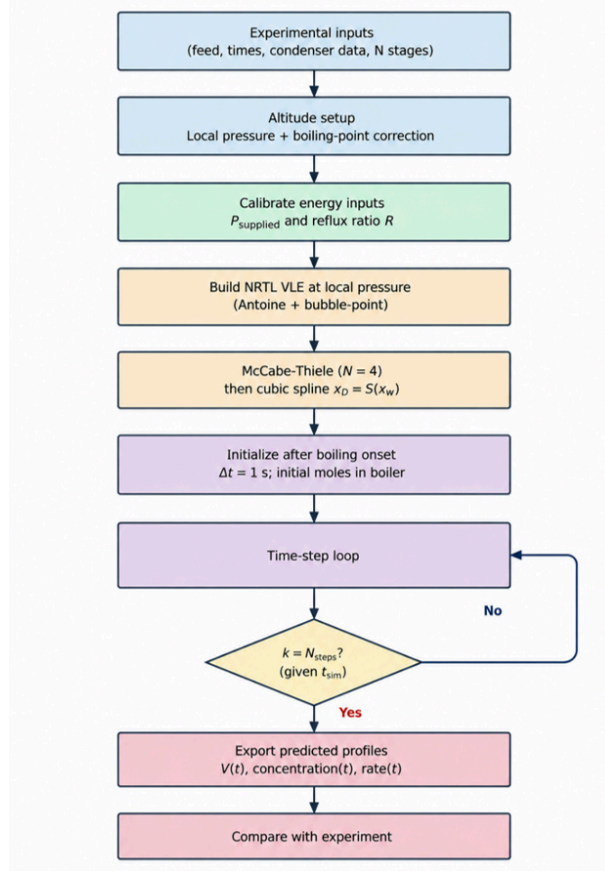
Figure 1. Flowchart of the NRTL batch-distillation solver: altitude-corrected VLE and energy estimation, McCabe–Thiele spline construction, and the 1-second time-stepping loop used to predict distillate volume and composition
